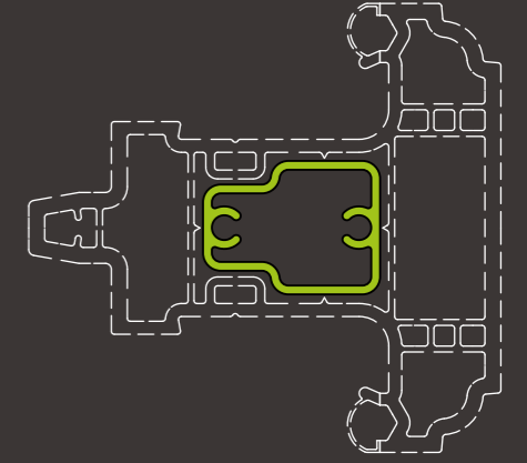
LFS212 80mm Flush Sash Transom Aluminium Reo
