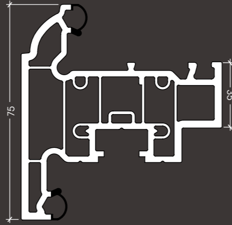
LFS031 80mm Flush Sash
