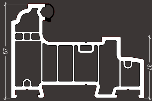
LFS011 80mm Flush Outer Frame
