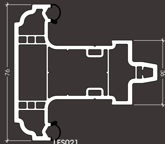
LFS021 80mm Flush Sash Transom T
