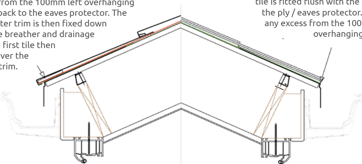
Metrotile/Extralight Section Showing Breather Membrane.
