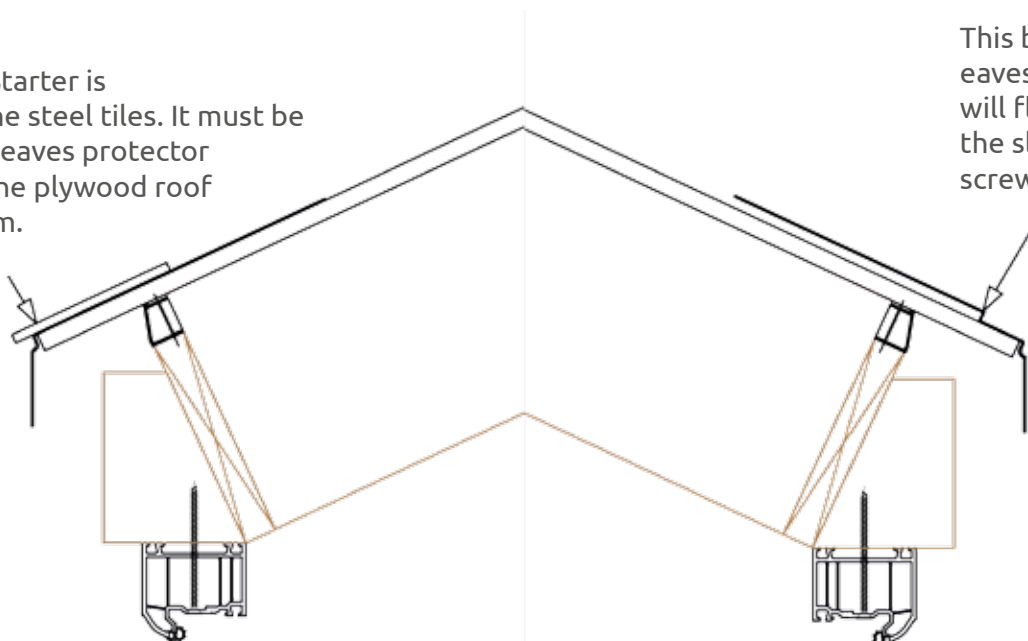
Metrotile Section Showing Eaves Protector Position.
