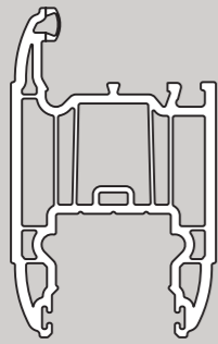
LPD082 Sash
